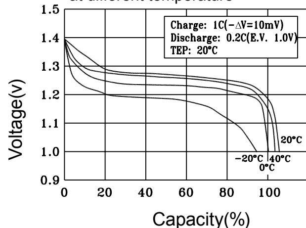
Discharge characteristics at different temperature
